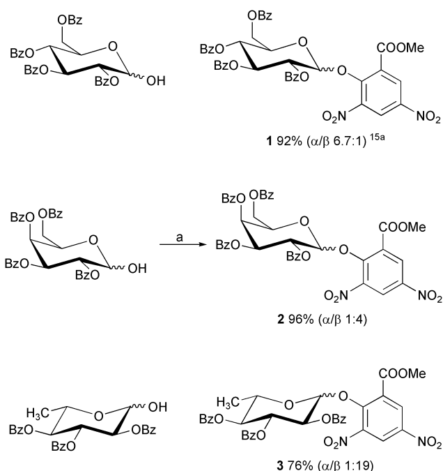
Scheme 1 Synthesis of glycosyl donors 1 (as recently reported 15a ), 2 , and 3 . a) Li 2 CO 3 , methyl 2-fluoro-3,5-dinitrobenzoate, DMAP, CH 2 Cl 2 .
